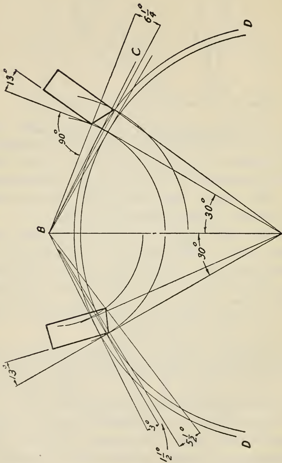
Figure 36. Equidistant pallets.
